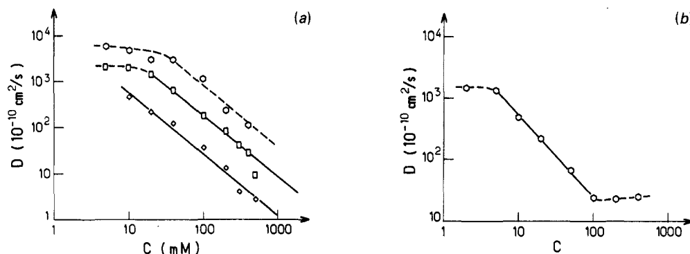
Figure 1. (a) Log-log plot of self-diffusion coefficient D_s versus lecithin concentration in isooctane solutions at 25 °C: \circ , w_0 = 0 ; \square , w_0 = 1 ; \diamond , w_0 = 2 . The full curves are least-squares fits; the broken curves are guides for the eye. The slopes for the full curves are -1.32 for w_0 = 1 and -1.35 for w_0 = 2 . (b) CTAB + 0.5 M KBr at 35 °C. The full curve is a least-squares fit. Its slope is -1.32 .
