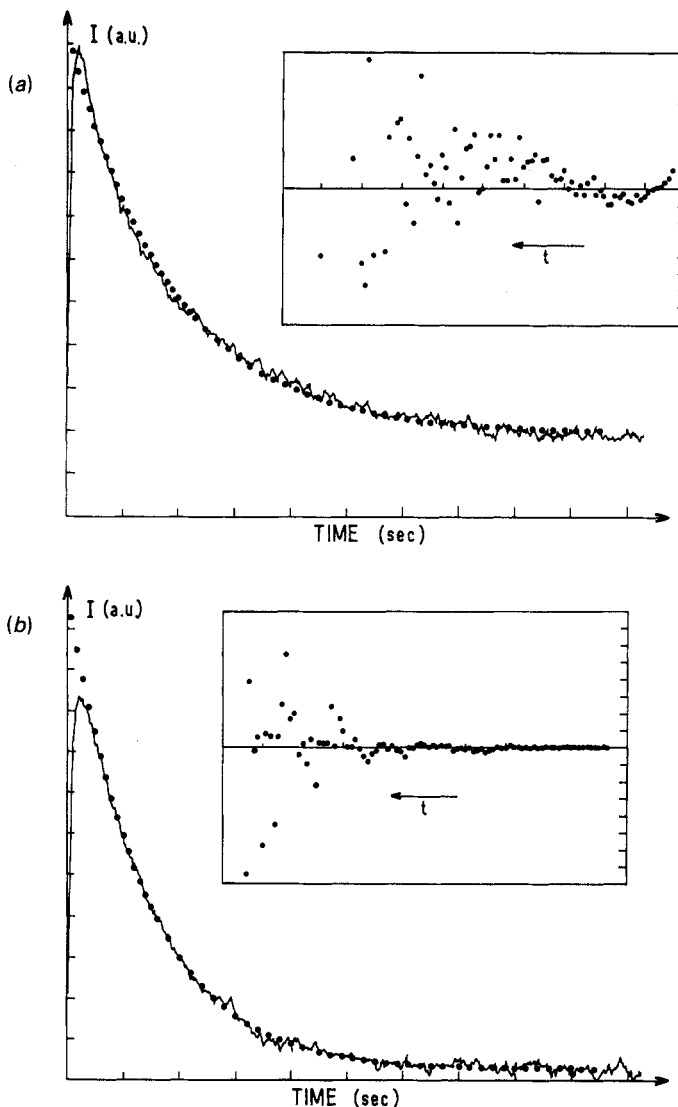
Figure 3. Typical decrease of the modulated fluorescence intensity (in arbitrary units) versus time. The curve is the experimental curve (the initial section where the signal increases with time is due to the finite response time of the lock-in amplifier). The dots represent the exponential fit. (a) Dilute sample. (b) Semidilute sample. Insets: plots of the residues (difference between experimental and theoretical curves). It is clear that the curve in (a) is non-exponential whereas the curve in (b) is exponential.
